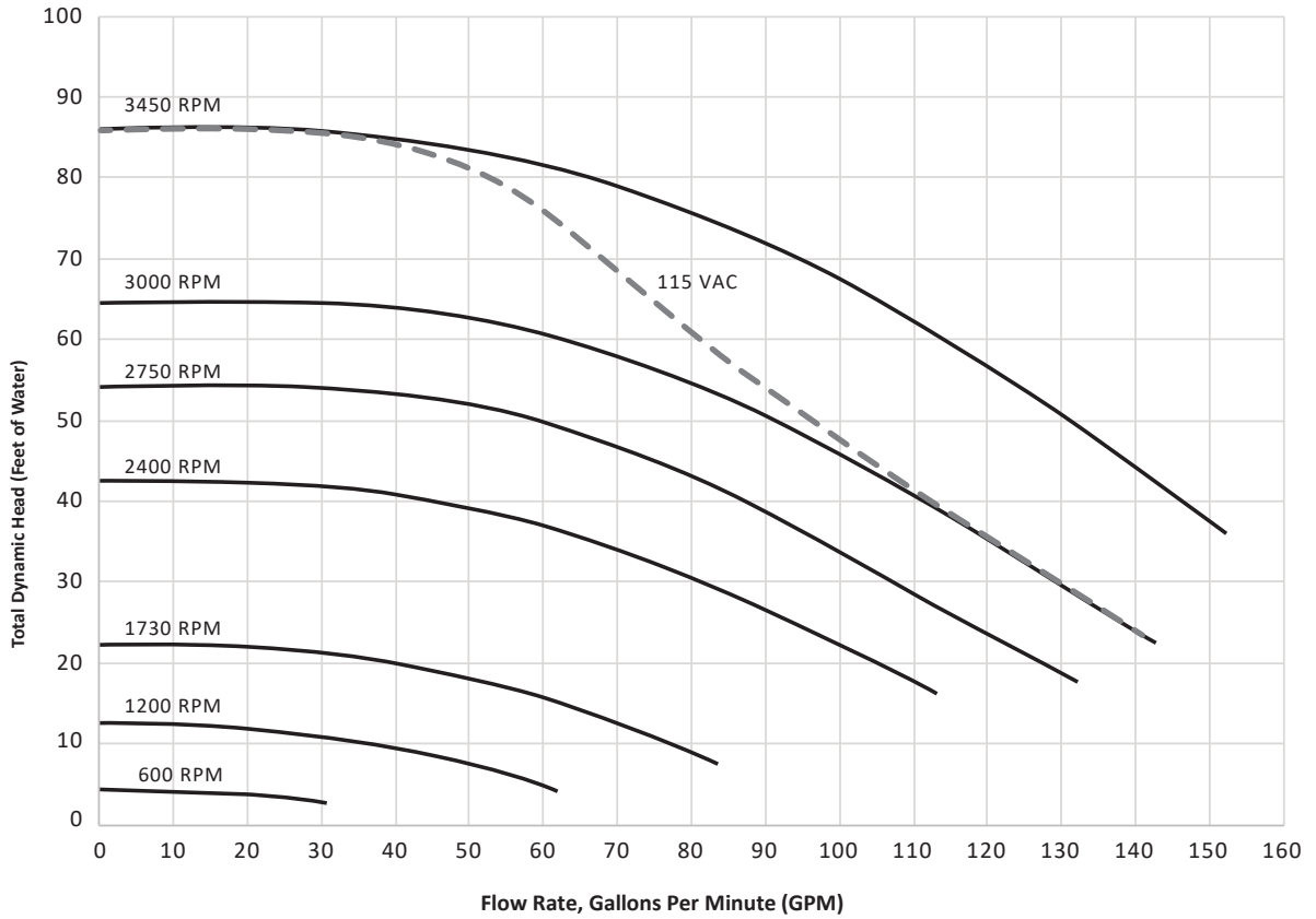
VSPHP270DV2A Performance Curves
