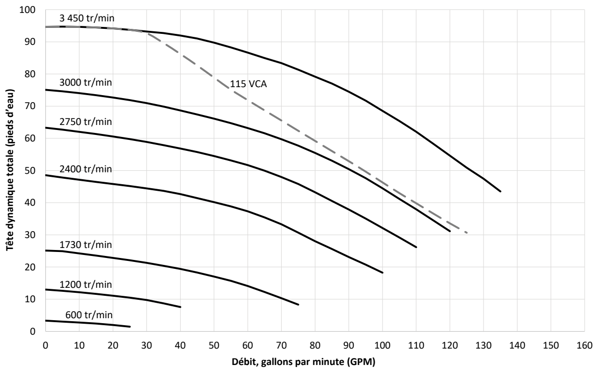
Courbes de performance VSFHP270DV2A
