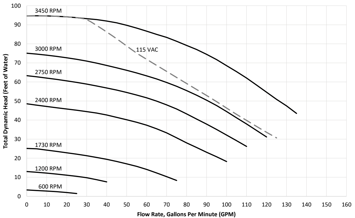
VSFHP270DV2A Performance Curves
