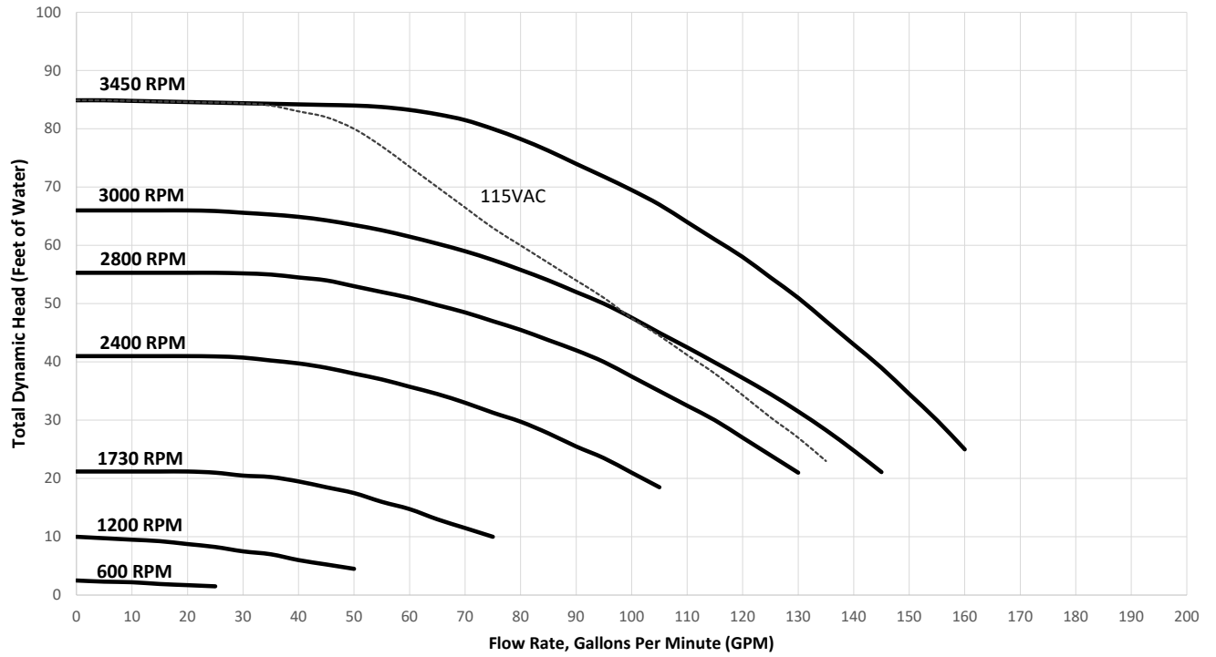
VSSHP270DV2A Performance Curves
