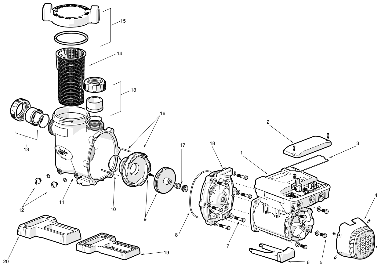
Figure 19. Jandy DV2A Model Variable Speed Pump Exploded View
