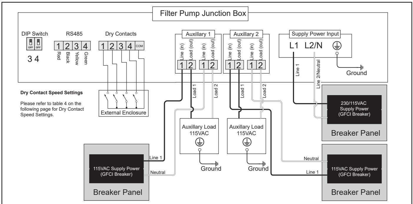
Figure 11. 115V Auxiliary Relay Wiring Diagram*
