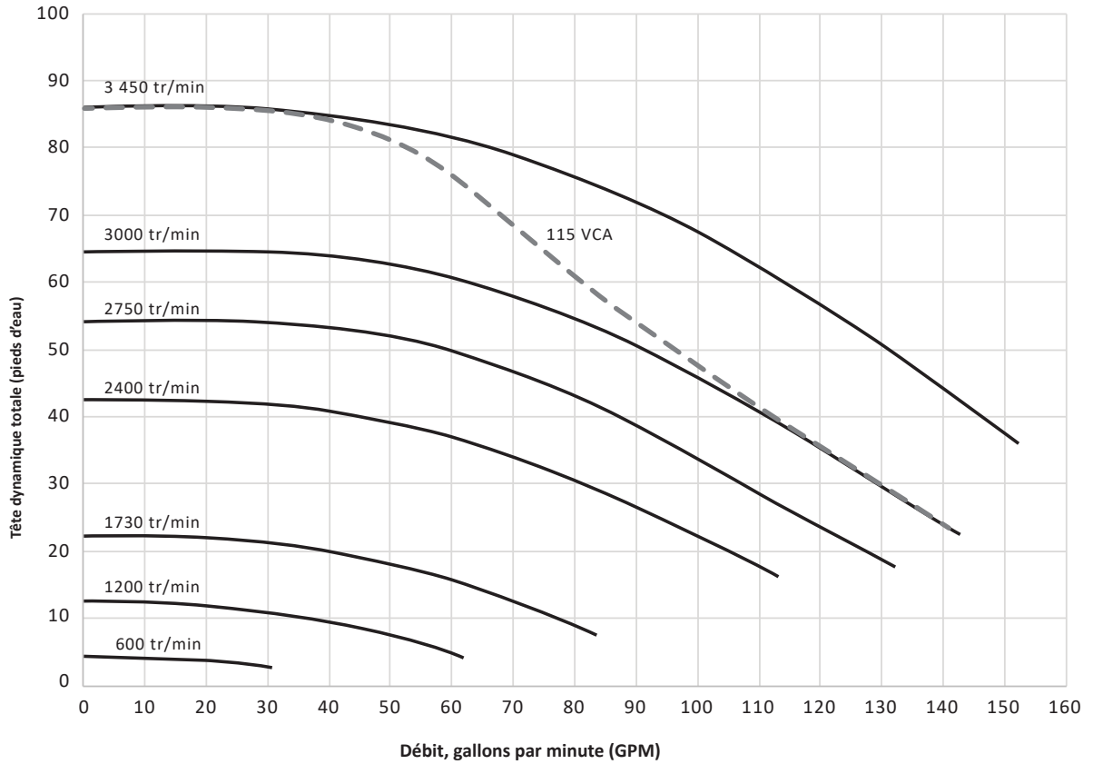
Courbes de performance VSPHP270DV2A
