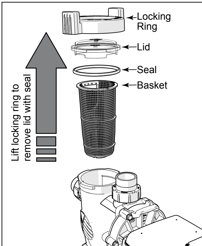
Figure 18. Remove Pump Lid
