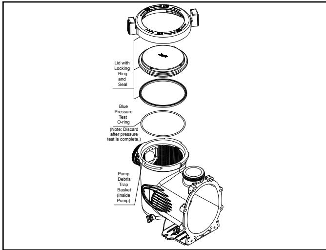
Figure 14. Exploded View with Blue Pressure Test O-ring (VSSHP Pump Models Only)
